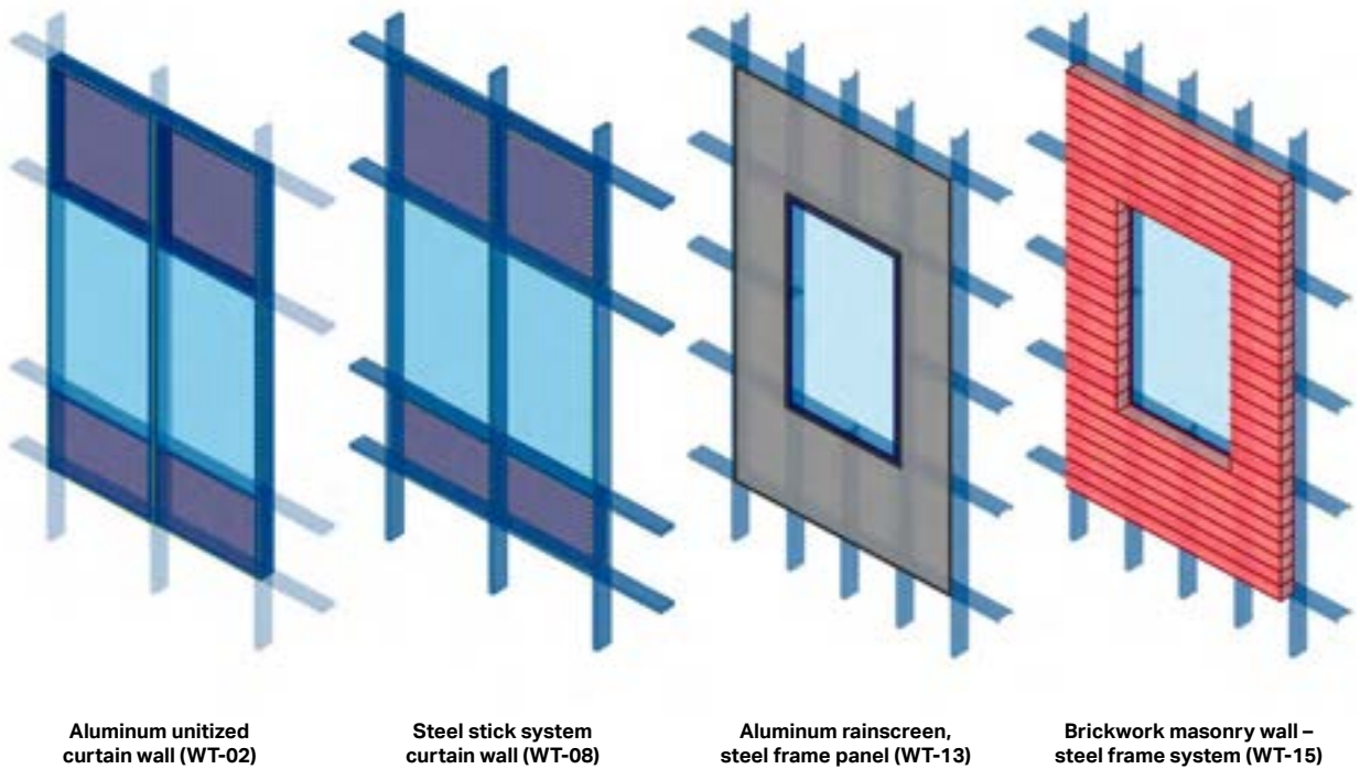
Figure 65: Façade typologies
