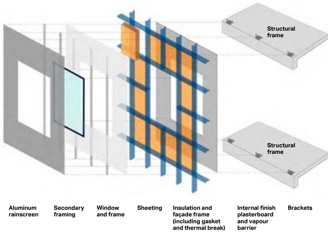
Figure 61: Aluminum rainscreen, steel frame panel (WT-13)
