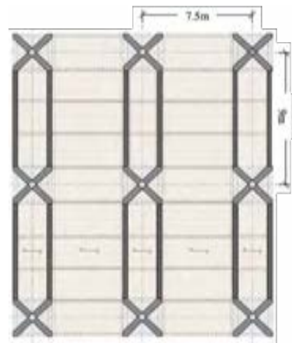
Figure 53: Hybrid reinforced concrete and timber frame proposal for an office building in London
