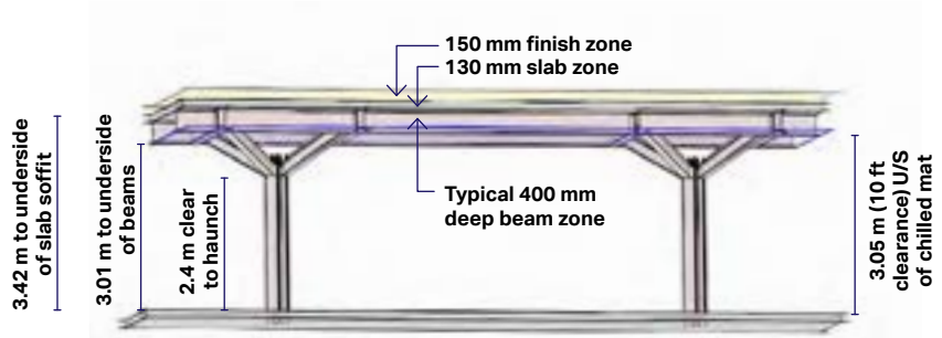
Figure 48: Tree column floor system developed by Make Architects and Arup – effectively shortening the span
